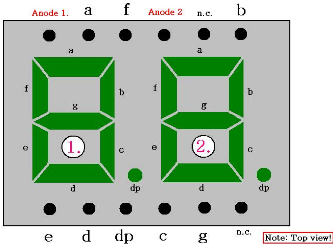
LTD-6402HG common anode 7 segments LED display
